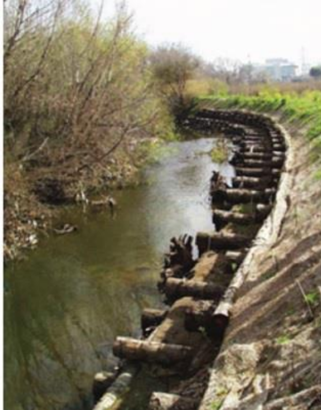
Flood protection
